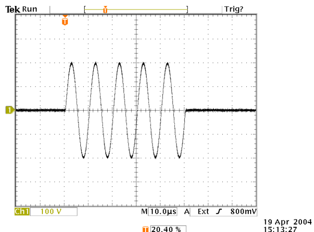
Waveform generated using burst mode option: Burst of 5 sine cycles, 100 kHz, 200V peak, to 1.2 kΩ. 100 V/div, 10 us/div.
